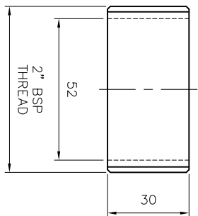
(SCALE-1:4) DETAIL-A BUSH FOR COUPLER
