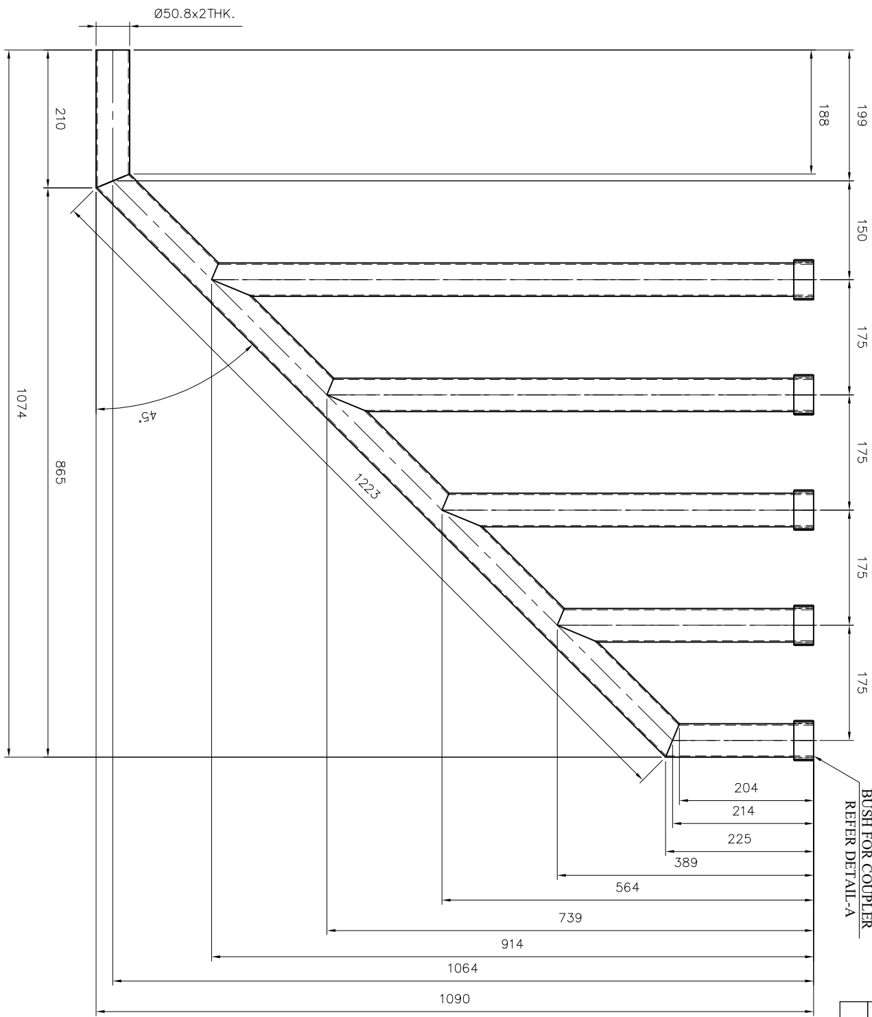
DETAIL OF BRANCH PIPE
